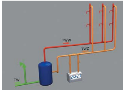
Fig.: Installation Sheme
