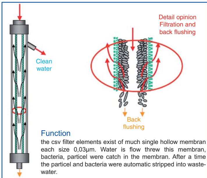
Illustration: BALS Filter
