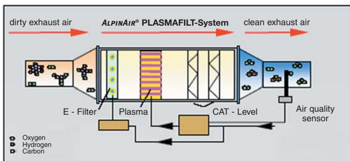
Fig.: ALPINAIR® PLASMAFILT System - exhaust air purification
